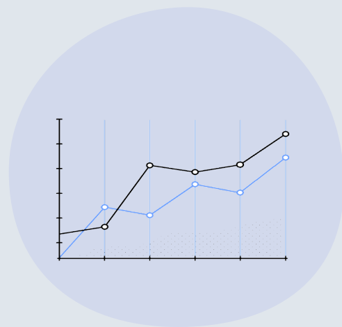
Mathematical Modelling
